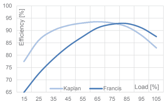
Fig. 2 Typical efficiency curves for Kaplan and Francis turbines
